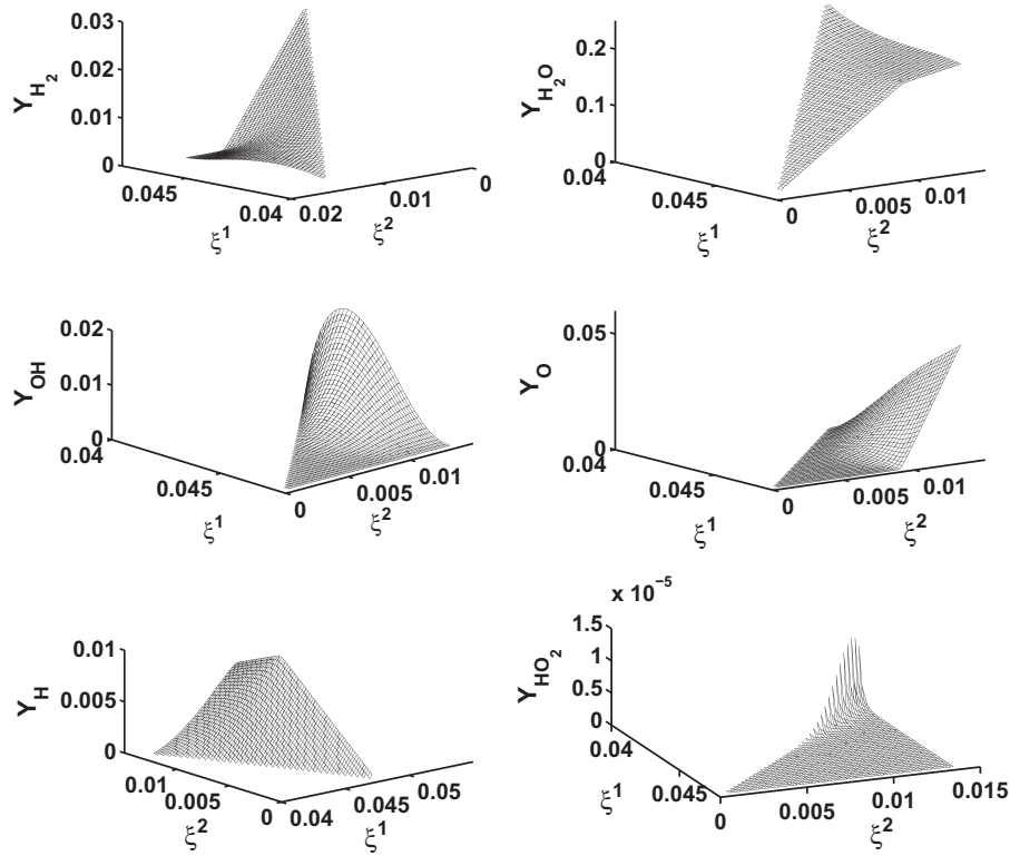
Fig. 1. 2-dimensional quasi equilibrium grid (QEG) for stoichiometric mixture of hydrogen and air, under p = 1 bar and \bar{h} = 2.8 kJ/kg. Six coordinates function of the parameters \zeta^1, \zeta^2 with \varepsilon_1 = \varepsilon_2 = 1.8 \times 10^{-4} .
