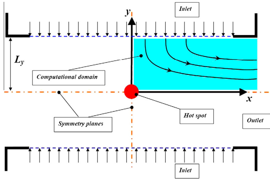
Fig. 5. Schematic representation of the 2-dimensional counterflow setup.
